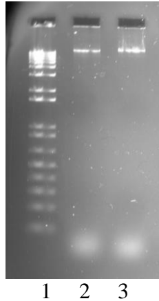
Figure 2.2 Gel image of DNA extraction products. Lane one contains a 1 kilobase (kb) ladder. Lane 2 contains 1 \mu L of DNA extraction product from Penicillium virginium . Lane 3 contains 1 \mu L of DNA extraction product from Aspergillus parasiticus SU-1.
