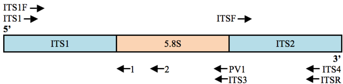
Figure 2.1 Primer annealing locations
