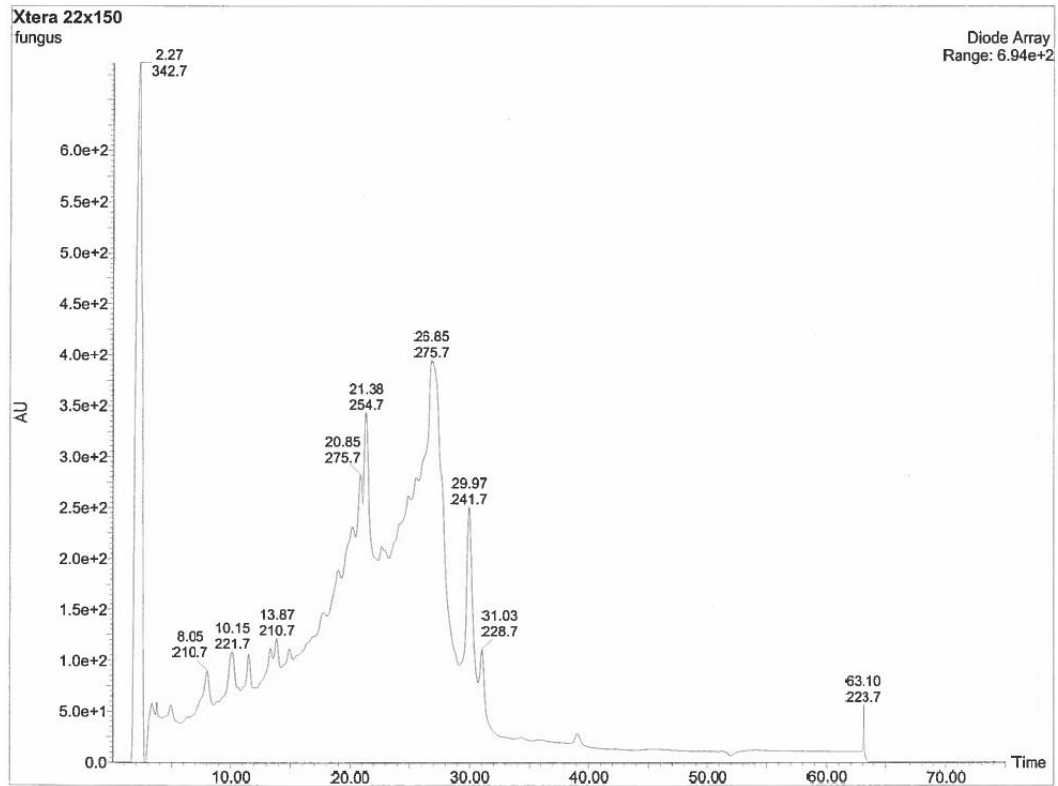
Figure 4.5 (A) Liquid chromatography chromatographs associated with the methanol fraction. The Y axis represents a given response from the instrument and the X axis represents the time of elution off of the LC column. The individual numbers above each represent the PDA signal (mas UV associated with the peak) and the nominal mass of the predominant ion under a given peak. Part A represents the reading collected during the entire 75 minute run and Part B represents the fractions collected during minutes 1-35.
