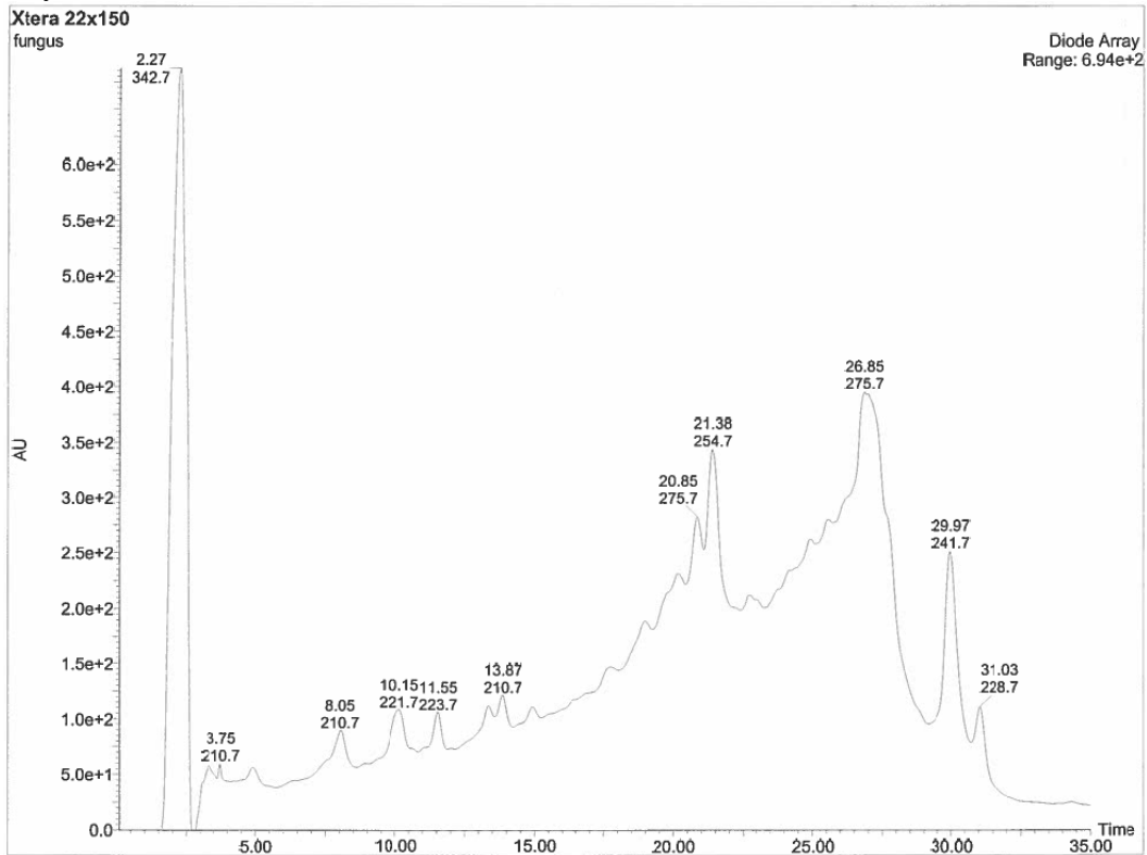
Figure 4.5 (B) Liquid chromatography chromatographs associated with the methanol fraction. The Y axis represents a given response from the instrument and the X axis represents the time of elution off of the LC column. The individual numbers above each represent the time of elution off of the LC column. The individual numbers above each represent the PDA signal (mas UV associated with the peak) and the nominal mass of the predominant ion under a given peak. Part A represents the reading collected during the entire 75 minute run and Part B represents the fractions collected during minutes 1-35.
