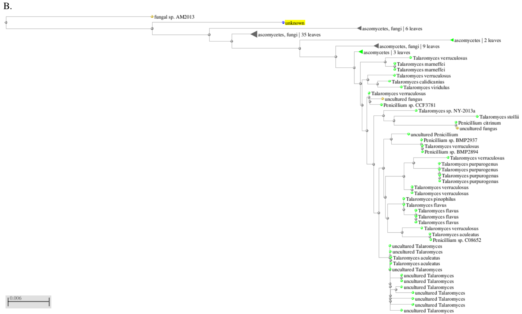
Figure 2.5 Neighbor Joining Tree generated from BLAST results of the ITS1-5.8S-ITS2 region of the rRNA gene of Penicillium virginium . Penicillium virginium is highlighted and label as unknown. B represents the 44 leaves not expanded at the bottom of A.
